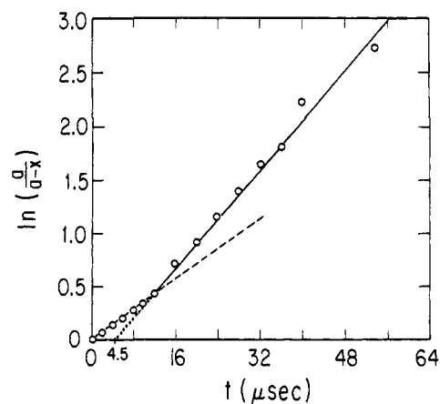
Figure 4. Pseudo-first-order rate plot for the formation of azobenzene from phenyl nitrene and phenyl azide. The concentration of azobenzene at time t is x ; the initial concentration of phenylnitrene and the final concentration of azobenzene are given by a . The slope of the initial and flatter portion is 3.67 \times 10^4 \text{ sec}^{-1} ; the slope of the longer and steeper portion is 4 \times 10^4 \text{ sec}^{-1} .
