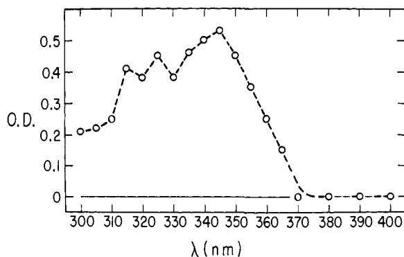
Figure 1. Absorption spectrum of 2-nitrenobiphenyl, taken 50 \mu\text{sec} after photolysis of 2-azidobiphenyl in cyclohexane. Units are optical density, to base 10.
