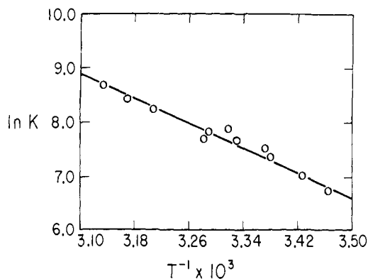
Figure 3. Arrhenius plot yielding activation energy of 11.46 \pm 0.76 kcal/mol for the formation of carbazole in cyclohexane solution.
