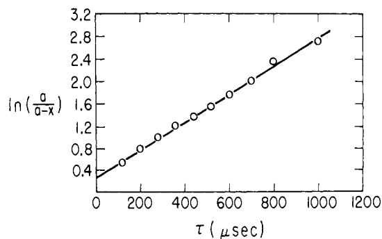
Figure 2. First-order rate plot for carbazole formation in cyclohexane at 340.0°K.
